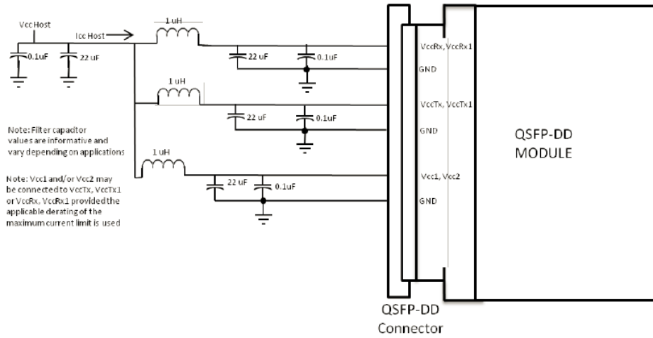
Figure 4: Recommended Host Board Power Supply Filtering
