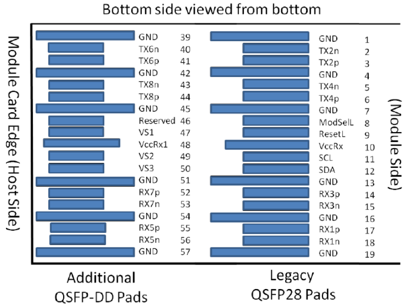
Figure 1: QSFDD Module pad layout
